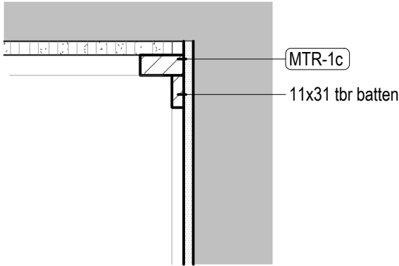
1 Cornice Typical 1 : 5
