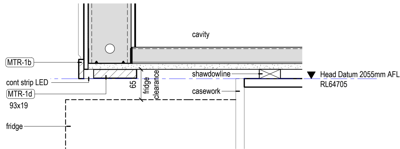
8 Kitchen Bulkhead 1 : 5
