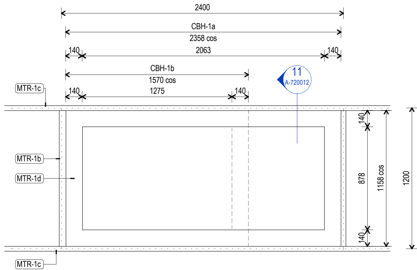
10 CBH-1 - Ceiling Acoustic Bulkhead 1 : 20 Plan Detail
