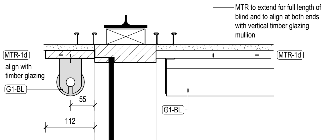
6 G1-BL 1 : 5 Blind & Ceiling - Interior
