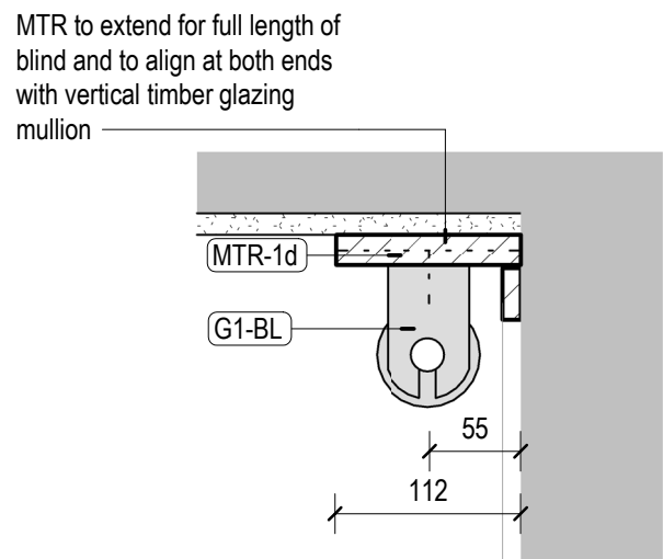
5 G1-BL 1 : 5 Blind & Ceiling - Exterior
