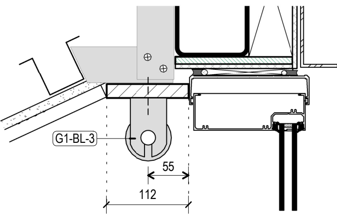
7 G1-BL-3 1 : 5 Blind & Raking Ceiling
