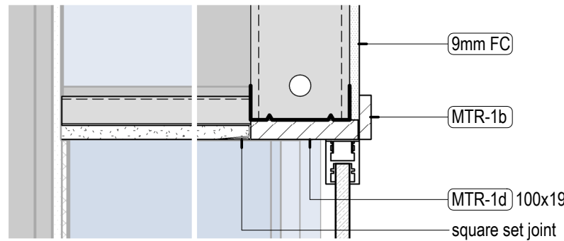
9 Bathroom Bulkhead 1 : 5
