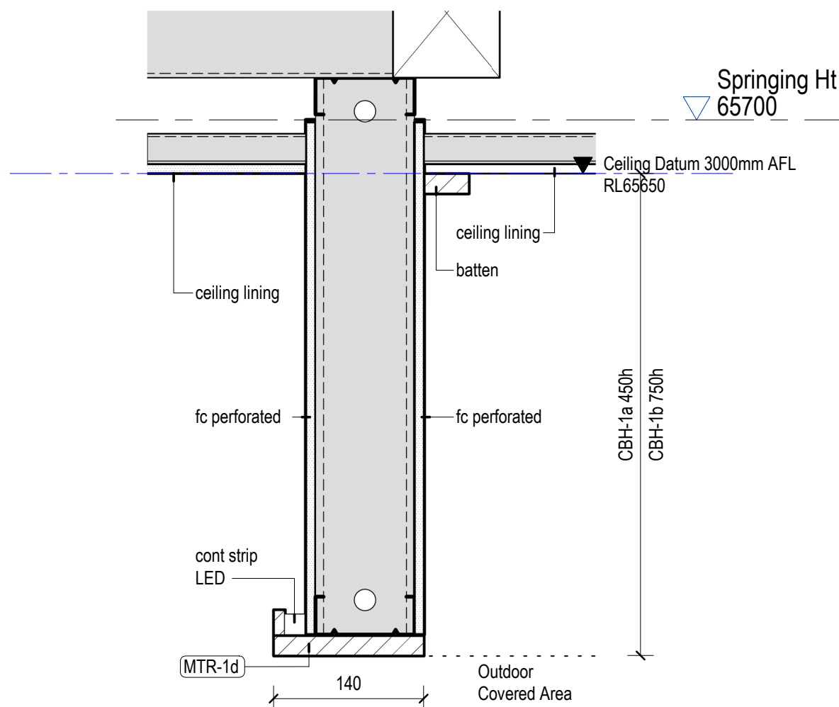
11 CBH-1 - Ceiling Acoustic Bulkhead 1 : 5 Detail Section
